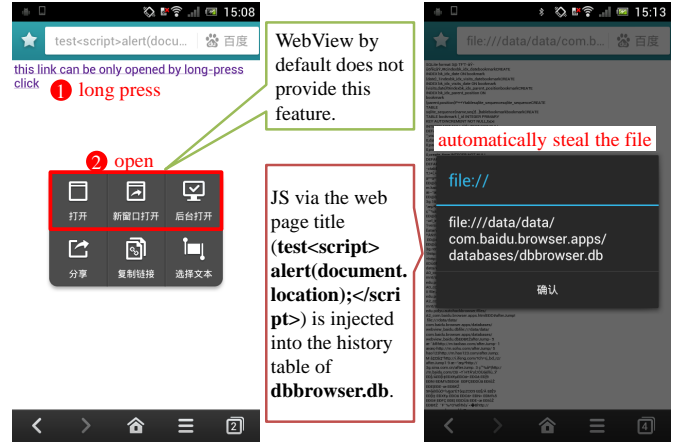
Fig. 3. An aimIFL-1 attack exploiting Baidu Browser.
